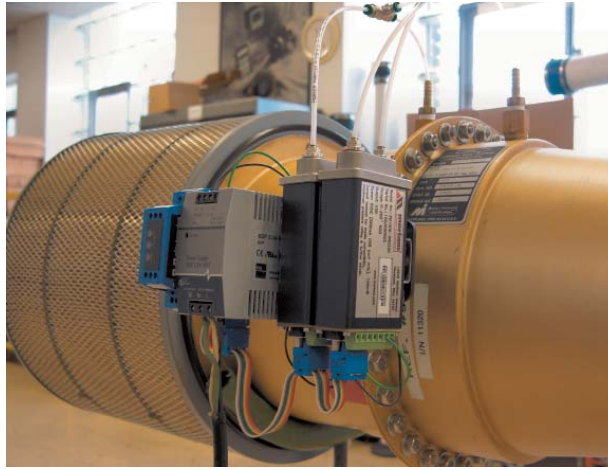
Meriam M1500 analog or digital transmitters for LFEs
